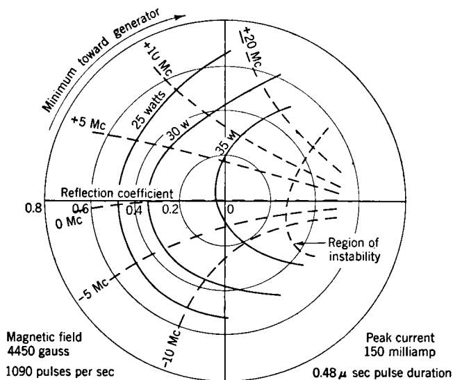
Frequency of 0 Mc contour = 9378 \text{ Mc/sec} FIG. 19-31.—Rieke diagram for BM50 magnetron.
